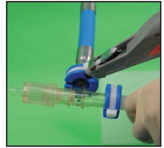
Finish closure by using SaniSure clamp tool to calibrated tension
